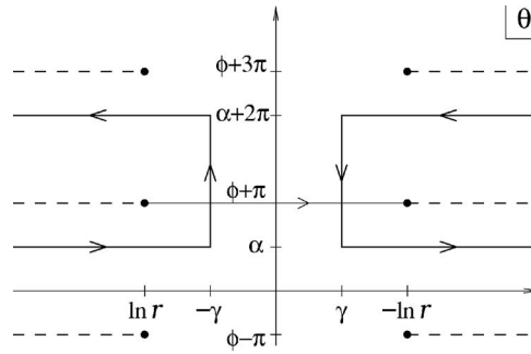
FIG. 1. Contours of integration in the \theta plane.
